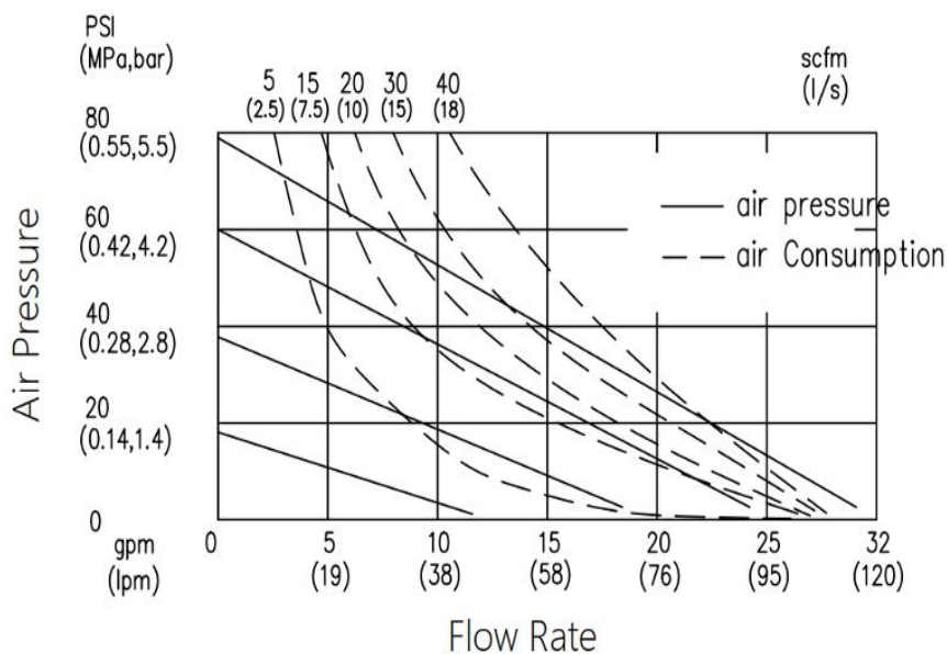
GK25 Technical Curve
