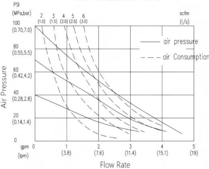
GK06 Technical Curve
