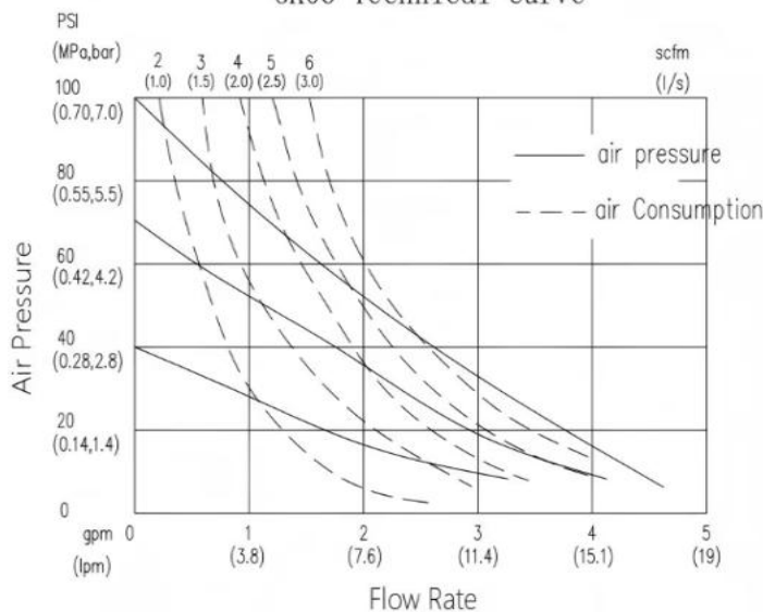
GK06 Technical Curve
