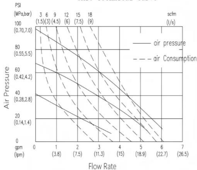
GK10 Technical Curve
