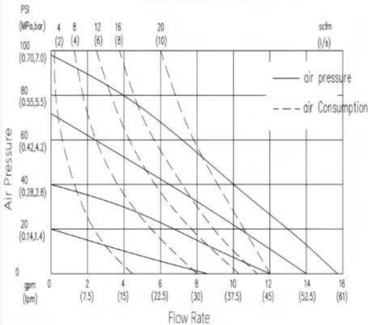
GK15 Technical Curve
