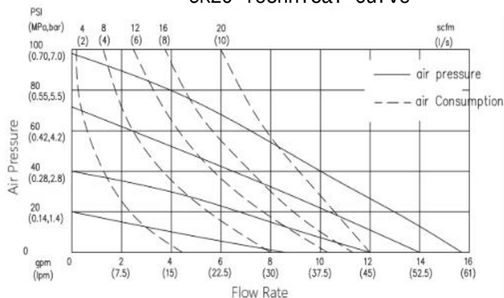
GK20 Technical Curve
