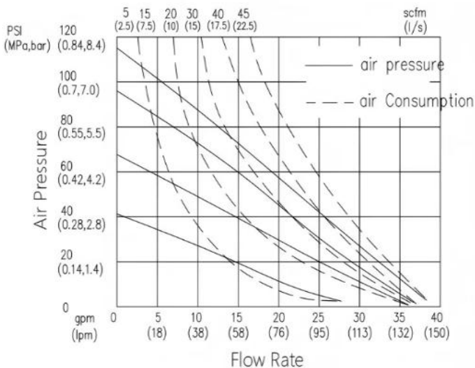
GK25 Technical Curve
