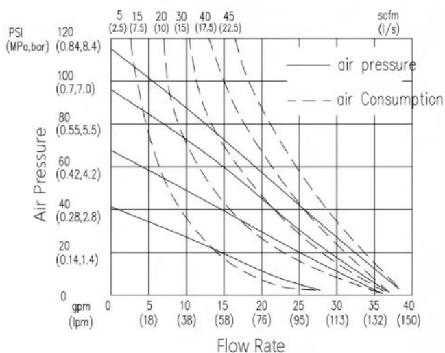
GK25 Technical Curve
