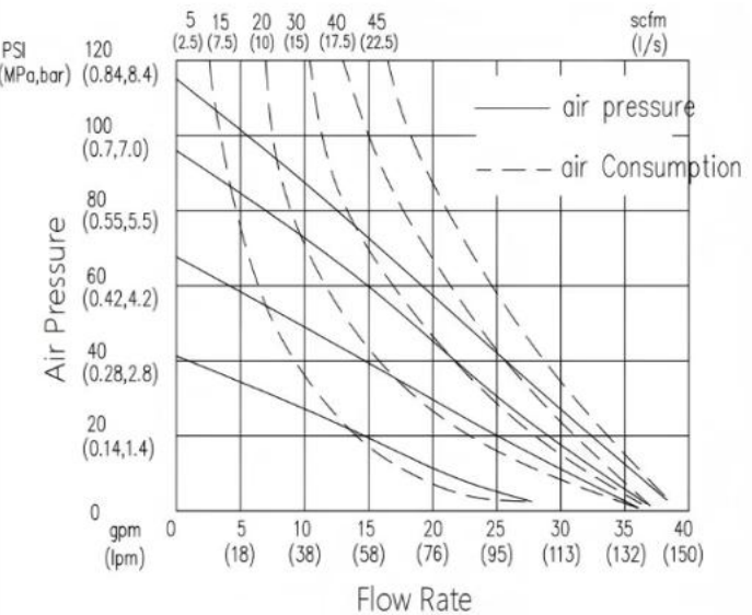
GK25 Technical Curve
