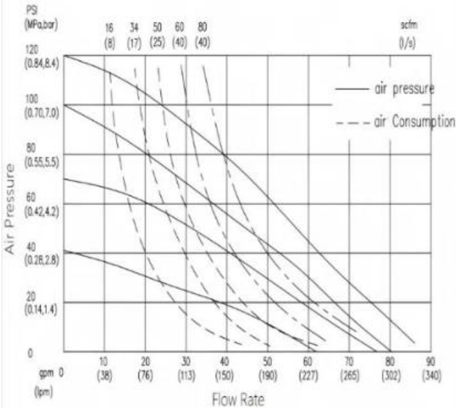
GK40 Technical Curve
