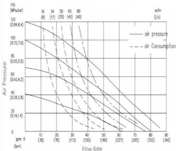
GK40 Technical Curve
