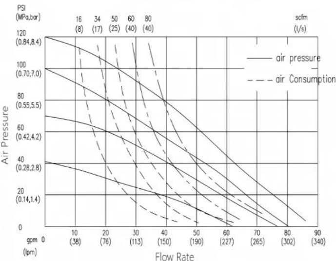
GK40 Technical Curve
