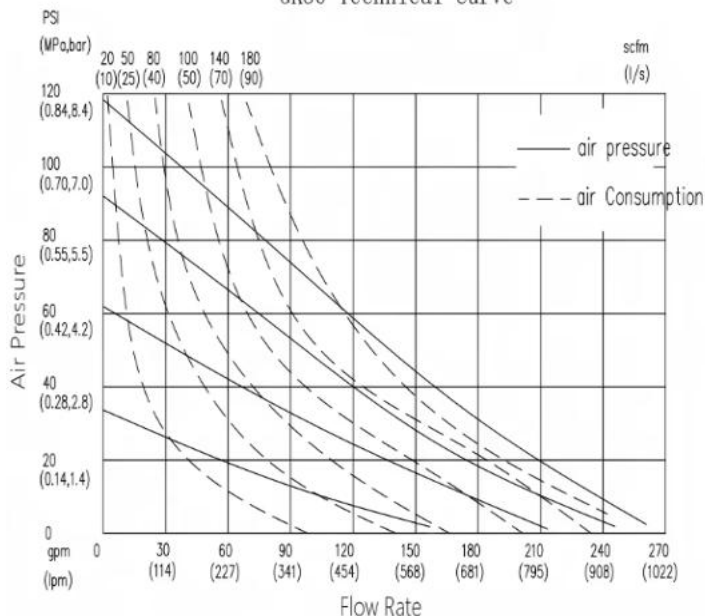
GK80 Technical Curve
