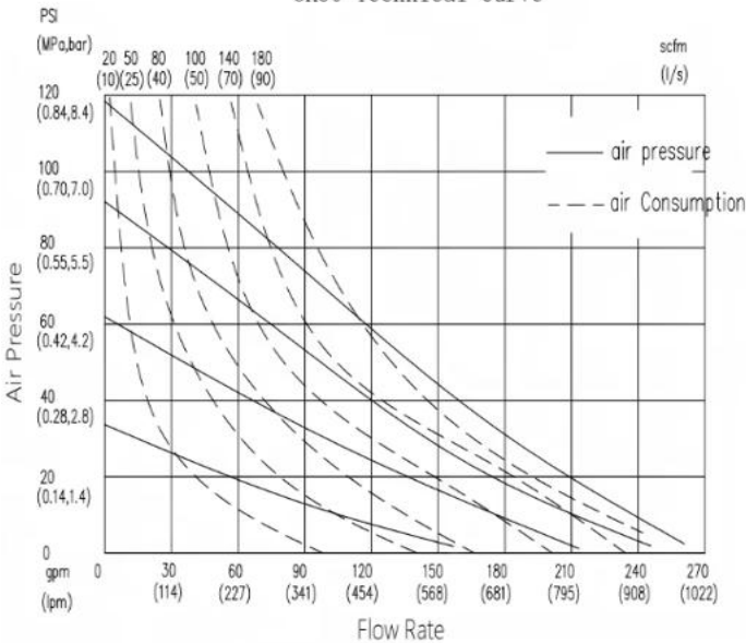
GK80 Technical Curve
