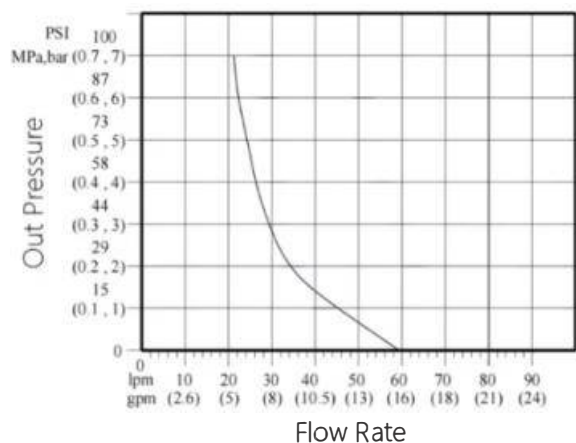
GKE25 Technical Curve
