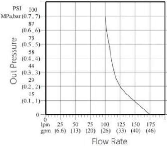
GKE50 Technical Curve
