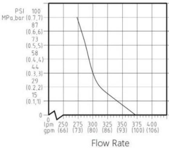
GKE80Technical Curve
